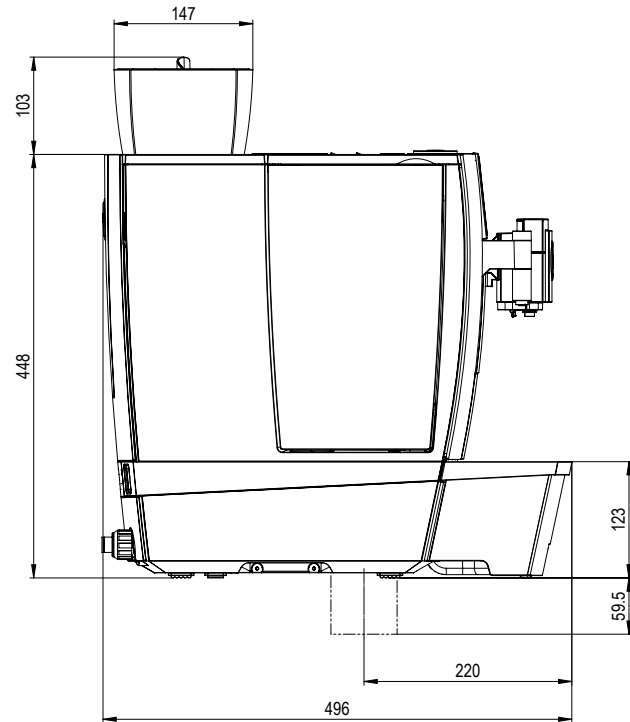
Side outline
